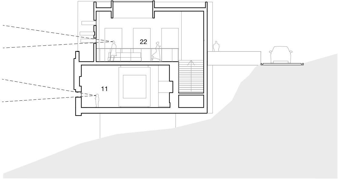
CC Section
